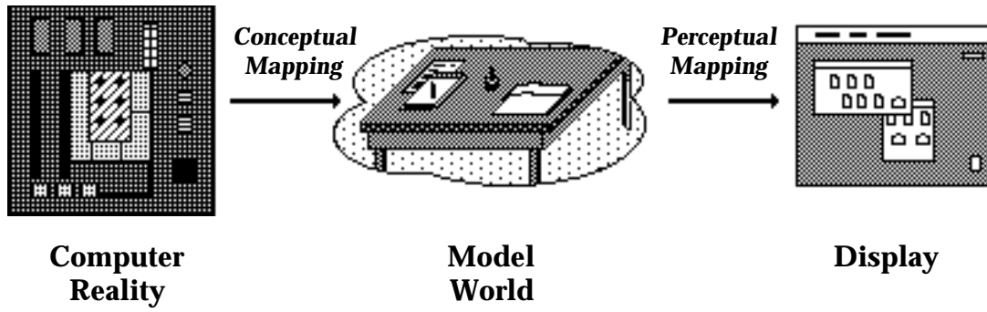
Figure 3. Two mappings exist between the reality of the computer and the display to which the user has access. The first is a conceptual mapping between events in the computer and those in some model world (for instance, that of a desktop). The second is a perceptual mapping between events in this model world and their perceptible manifestations, be they visual or auditory.
